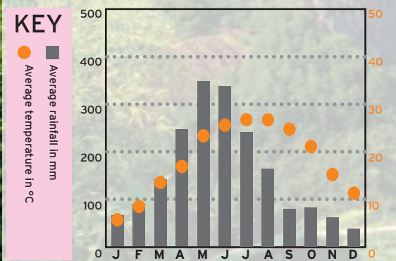
Guilin Climate Chart
