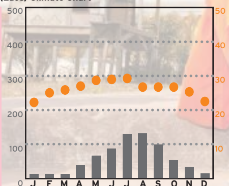
Vientiane (Laos) Climate Chart
